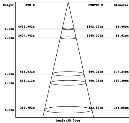
Parameter of DL-LW25/DL-LB25 | CCT 4000K
